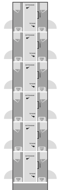
FLOOR PLAN
