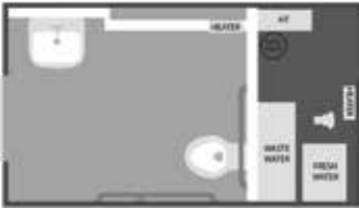
6'x11' | ADA, 1-STATION FLOOR PLAN
