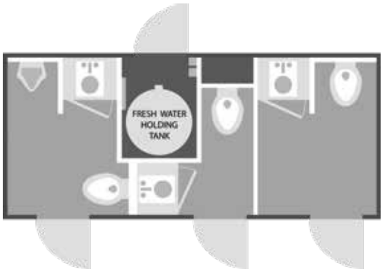
6x14' | 3-DOOR, 3-STATION FLOOR PLAN
