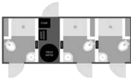
6x18' | 3-STATION, SHOWER COMBO FLOOR PLAN
