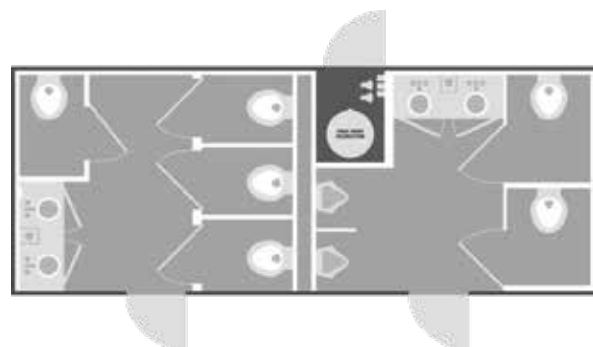
8x21' | 8-STATION FLOOR PLAN
