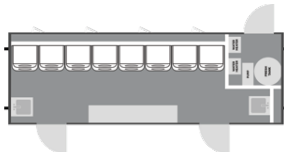
8x25' | 8-STATION, LAUNDRY FLOOR PLAN
