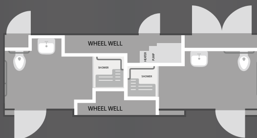
8x26' | ADA 2-STATION COMBO FLOOR PLAN
