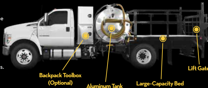
Aluminum Tank
